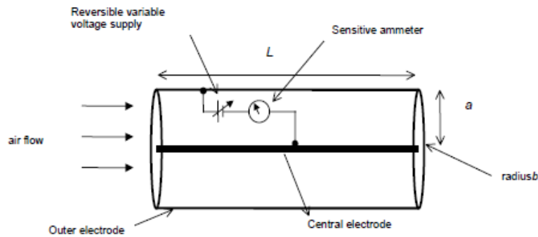
Figure 15 Illustration of the Gerdien condenser. [47]
