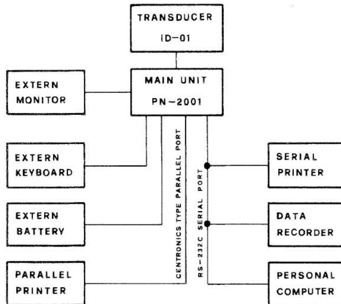
Figure 18 System configuration of PN-2001 ion meter.
