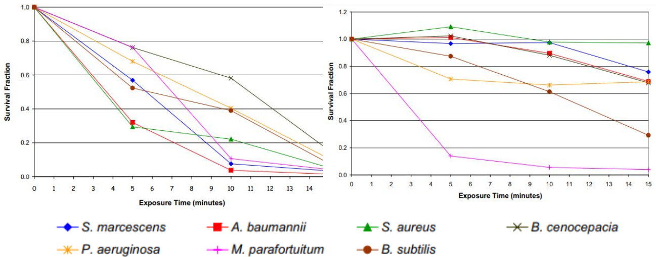
Figure 3 Bactericidal effect due to exposure to negative (on the left) and positive (on the right) ions. [26]
